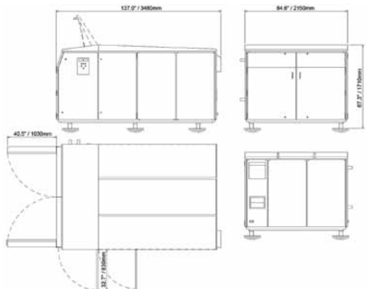
APV 185Q - BASE OUTLINE DRAWING
