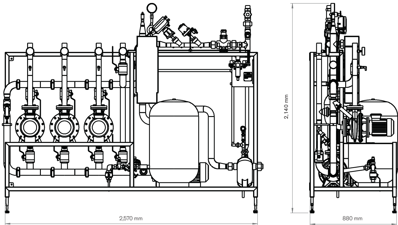
GS hot water unit with four loops
